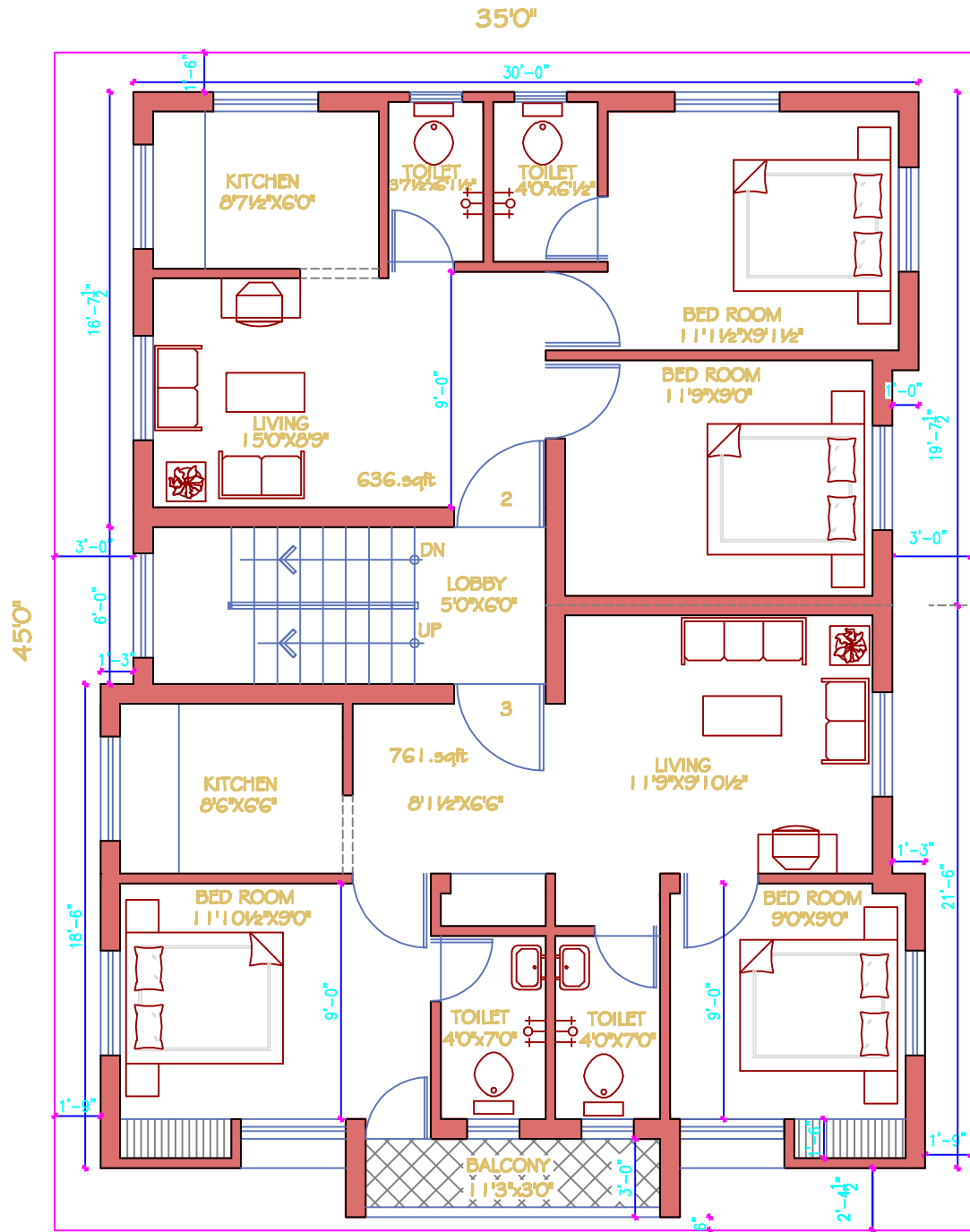
SITE CUM FIRST FLOOR PLAN
